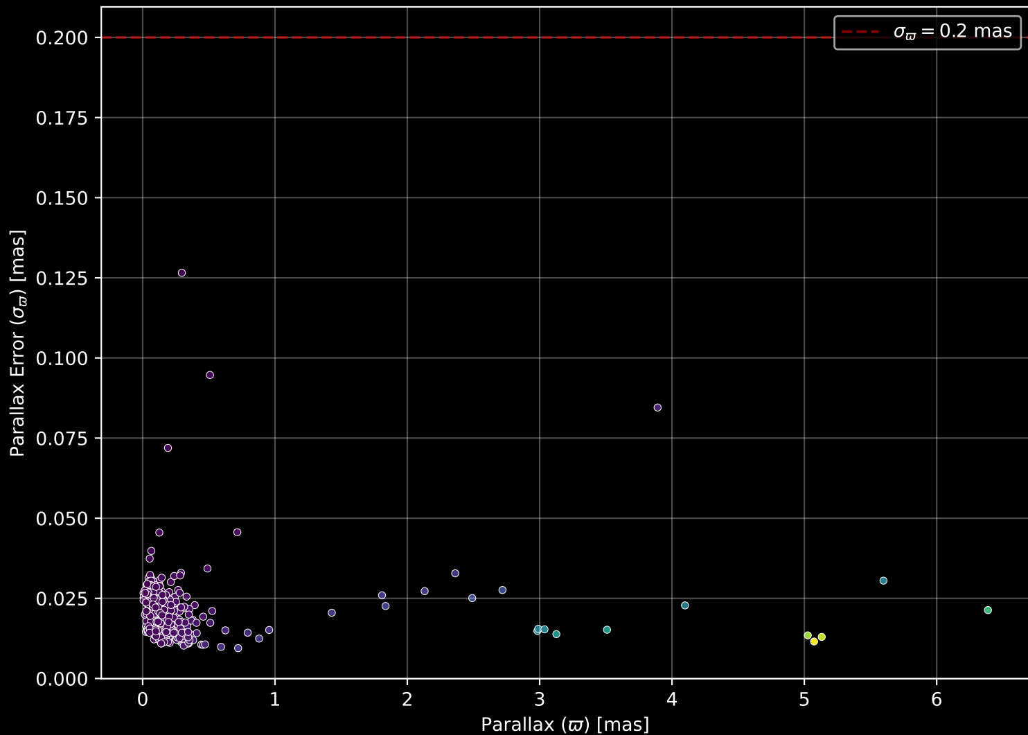
APOGEE DR17 Field: [064+06] Parallax Quality (n= 430)
