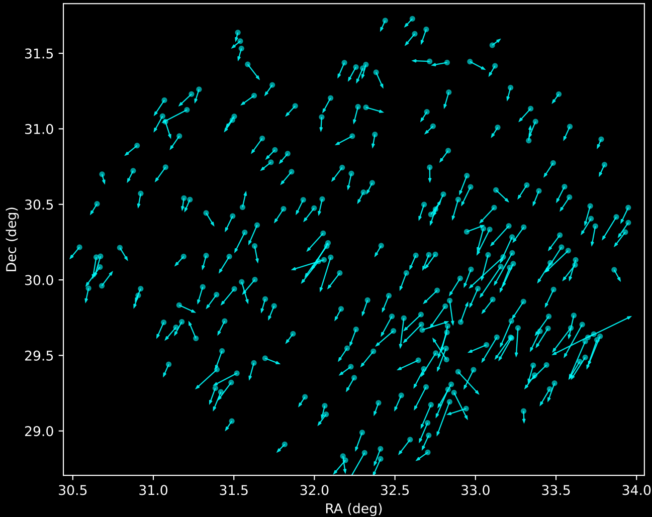
APOGEE DR17 Noise Stream Proper Motion Vectors (n=246)
