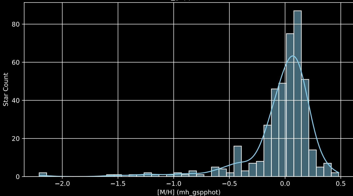
APOGEE DR17 Field: [064+06 [M/H] (mh_gspphot) (n= 425)
