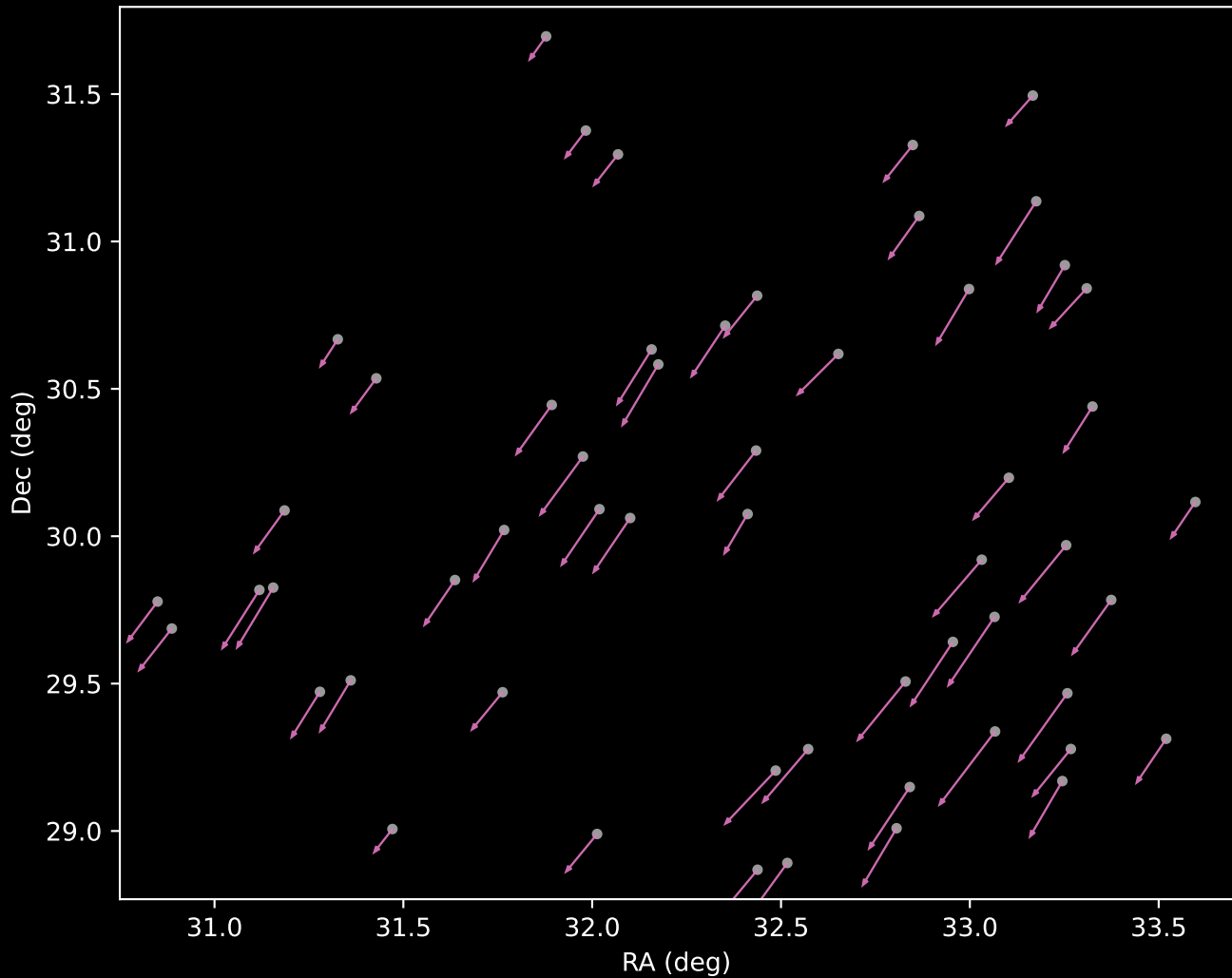
APOGEE DR17 Cluster 12 Proper Motion Vectors (n=55)
