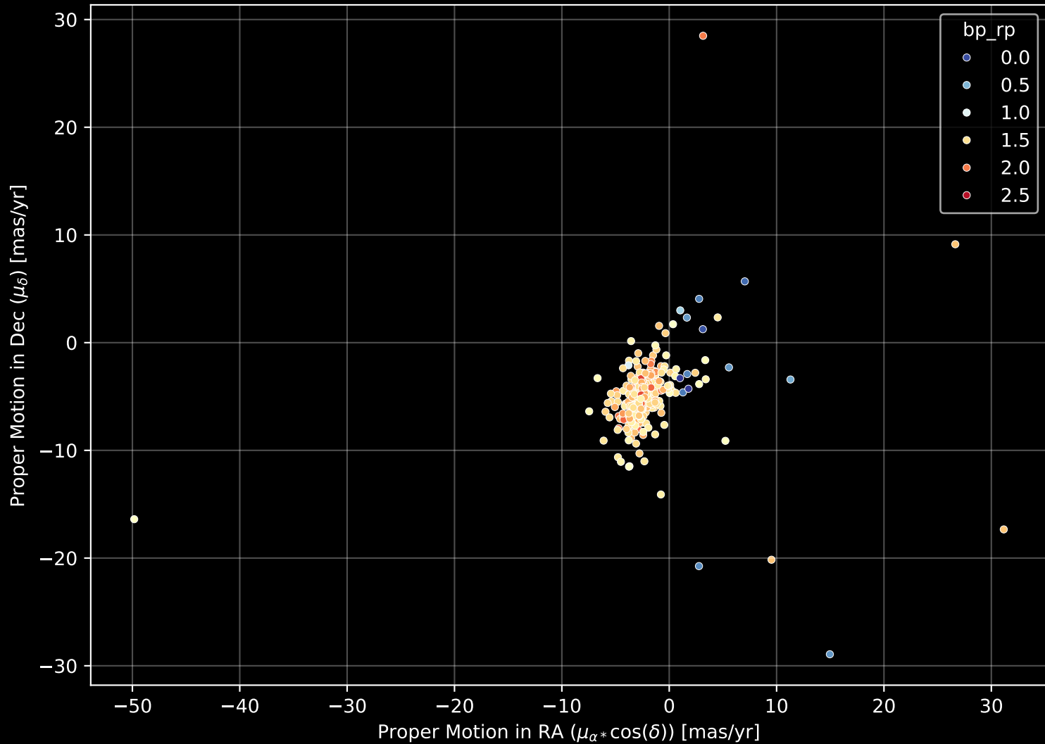
APOGEE DR17 Field: [064+06] Proper Motion Diagram (n= 430)
