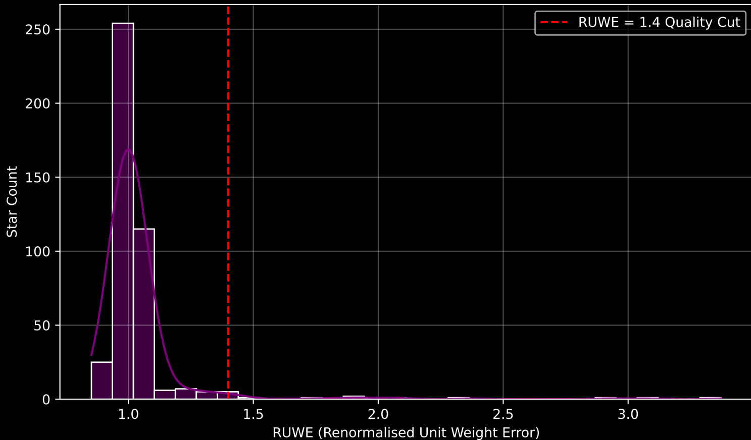
GAPOGEE DR17 Field [064+06] RUWE Distribution (n= 427)
